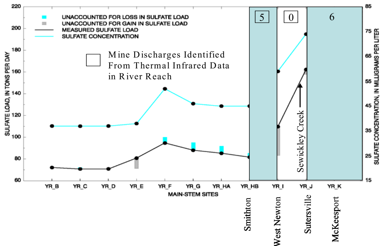
Figure 8. Mine drainage sites identified from TIR data and their relative location within river reach section of the lower Youghiogheny River, showing the effects of sulfate loads and concentrations
